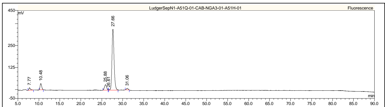
Figure 1 : LudgerSepN1 HPLC profile of 2AB labeled NGA3 glycan (Cat. #: CAB-NGA3-01, Lot No. A51H-01).
