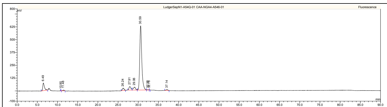
Figure 1 : LudgerSepN1 HPLC profile of 2AA labeled NGA4 glycan (Cat. #: CAA-NGA4-01, Lot No. A546-01).
