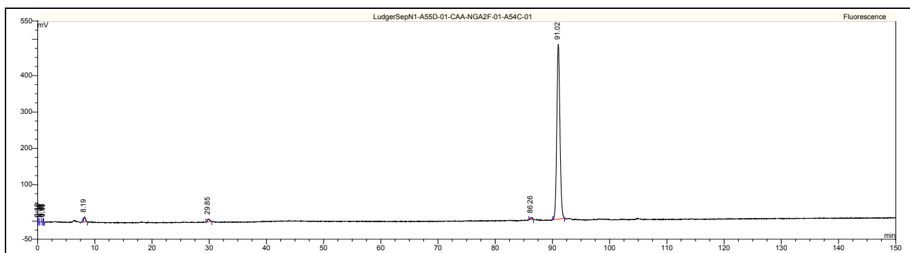
Figure 1 : LudgerSepN1 HPLC profile of 2AA labeled NGA2F glycan (Cat. #: CAA-NGA2F-01, Lot No. A54C-01).
