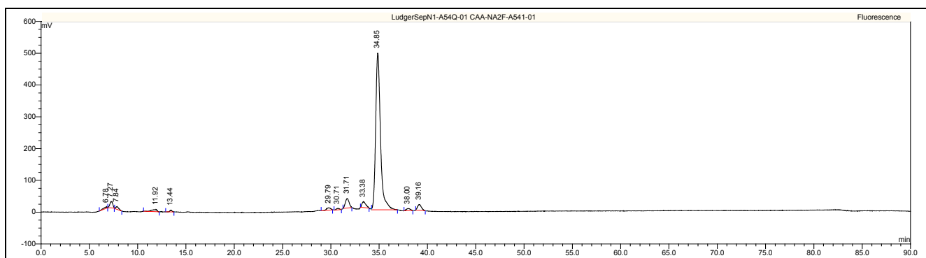
Figure 1 : LudgerSepN1 HPLC profile of 2AA labeled NA2F glycan (Cat. #: CAA-NA2F-01, Lot No. A541-01).
