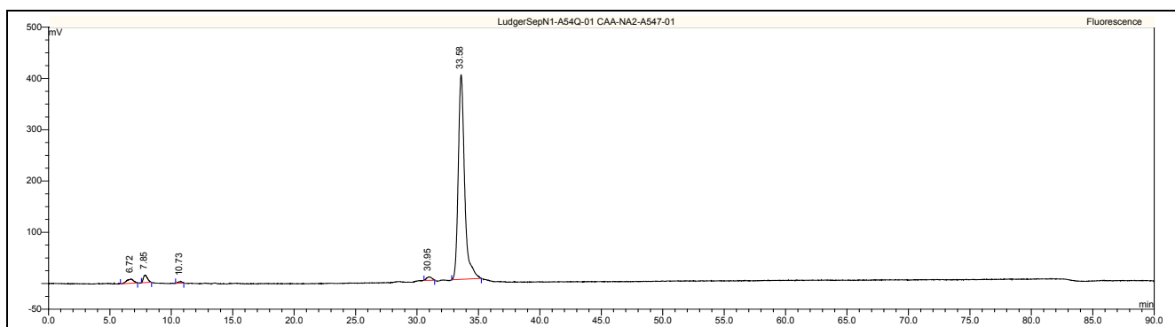
Figure 1 : LudgerSepN1 HPLC profile of 2AA labeled NA2 glycan (Cat. #: CAA-NA2-01, Lot No. A547-01).
