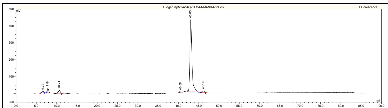
Figure 1 : LudgerSepN1 HPLC profile of 2AA labeled MAN-9 glycan (Cat. #: CAA-MAN9-01, Lot No. A53L-02).
