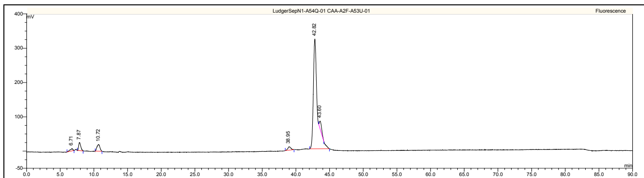
Figure 1 : LudgerSepN1 HPLC profile of 2AA labeled A2F glycan (Cat. #: CAA-A2F-01, Lot No. A53U-01).
