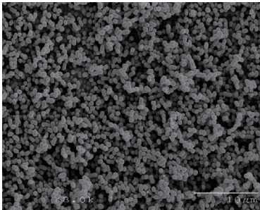
Figure 1. Electron micrograph of Leuconostoc mesenteroides 180720-12-1 strain
