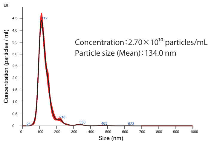
Figure 2. Particle size distribution of EVs derived from Leuconostoc mesenteroides 180720-12-1 strain
