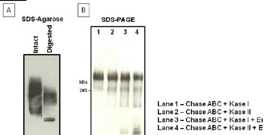
Fig.1 Western blotting of purified human cartilage aggrecan. (A) SDS-Agarose gel electrophoresis (0.5%) before and after combined chondroitinase ABC digestion of aggrecan (B) SDS-PAGE on 3-8% linear gradient gels, after the combined digestions of aggrecan indicated in the legend below.
