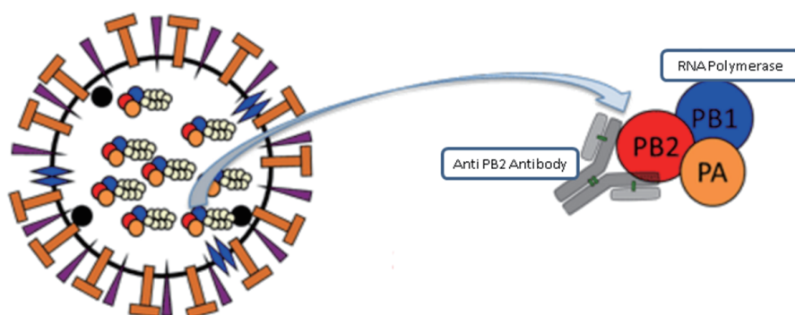
Depiction of Anti PB2 (clone# 3-1.6) and RNA Polymerase interaction.
