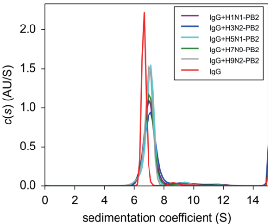
Figure 2. Ultracentrifugation analysis of IgG, PB2 (H1N1, H3N2, H5N1, H7N9, H9N2) + IgG
