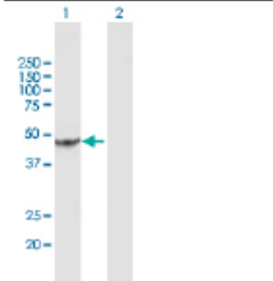
Western Blot analysis of ACAD8 expression in transfected 293T cell line by ACAD8 rabbit polyclonal antibody.
