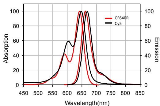
Figure 1. Absorption and emission spectra of CF™640R and Cy™5.
