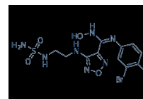
Chemical structure of Epacadostat (INCB024360)
