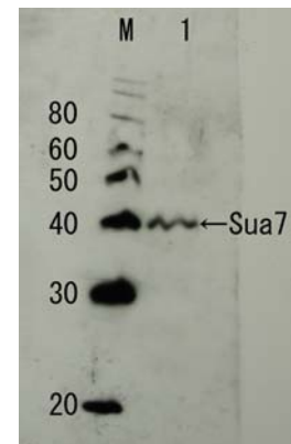
Fig. 1 Detection of Sua7p by Western blotting using the Sua7p antibody.
