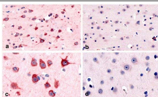
Immunohistochemistry on normal human brain cortex. The large neurons are strongly reactive. a)abx20 b)non-immune controlx20 c)abx40 d)controlx40.
